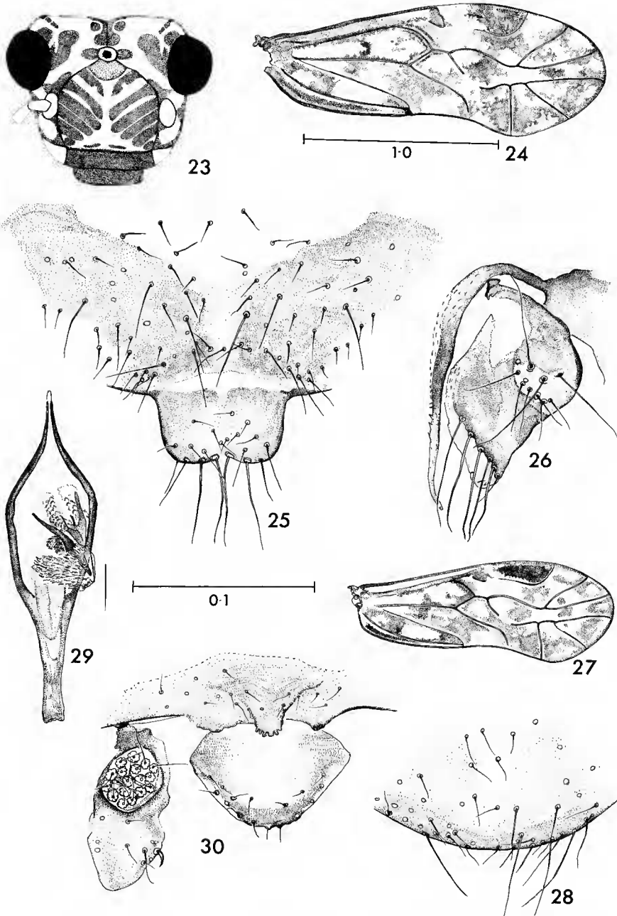
FIGS 23-30. — Peripsocus stegeri , ♀ holotype : 23, head; 24, fore wing; 25, subgenital plate; 26, gonapophyses. ♂ allotype : 27, fore wing; 28, hypandrium; 29, phallosome; 30, epiproct and paraproct. (Figs 24 and 27, and figs 25, 26 and 28-30, to common scales; fig. 23 not to scale.)
